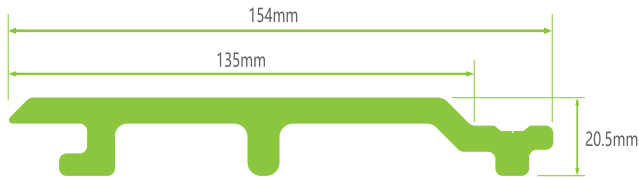
Model:S15420.5-3D
