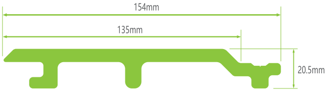
Model:S15420.5-G2
